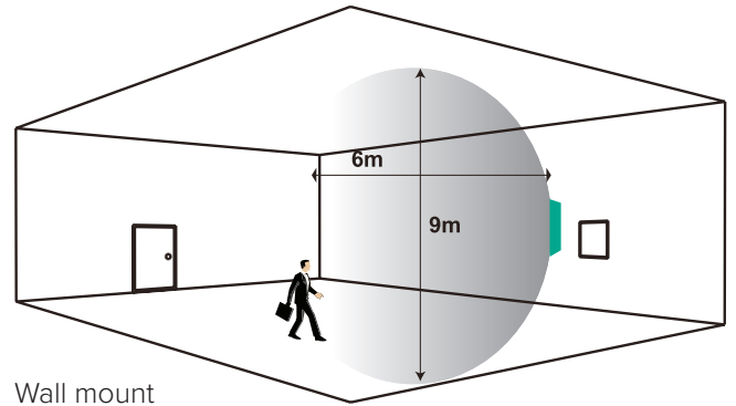
Wall mount
